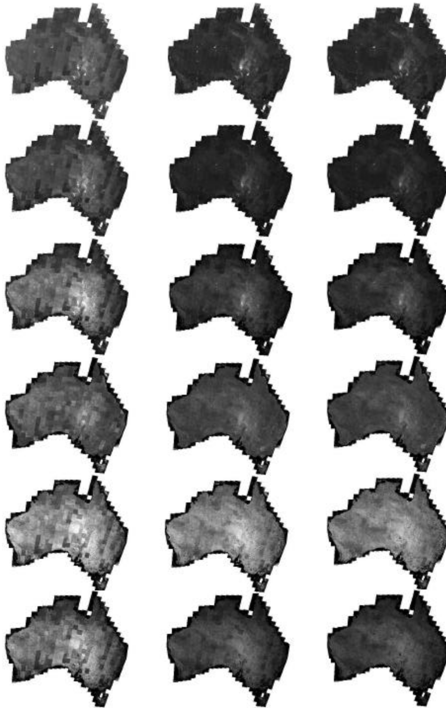
Fig. 1. Landsat 7 Mosaics of the Australian Continent.
