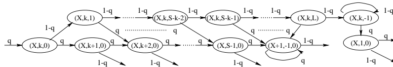
Figure 5. State Transition of Closing Operator, Large Success Run Lengths
