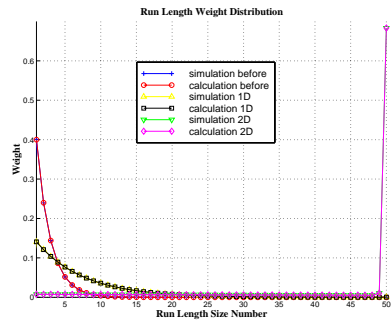
Figure 7. Run Length Weight Distribution
