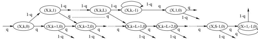
Figure 4. State Transition for Closing Operator, Small Lengths
