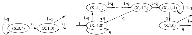
Figure 3. State Transition for Closing Operator, Initial condition for Success Runs (Left); Success Run Length Overflow (Right)
