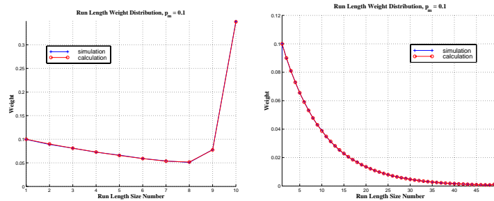
Figure 6. Run Length Weight Distribution, 1D
