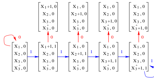
Figure 2. Diagram of Run Length Statistics Calculation Example
