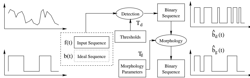
Figure 1. System Diagram
