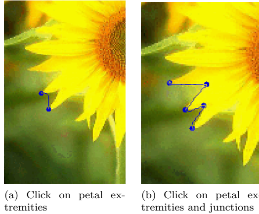
Figure 4. Intelligent scissors.
