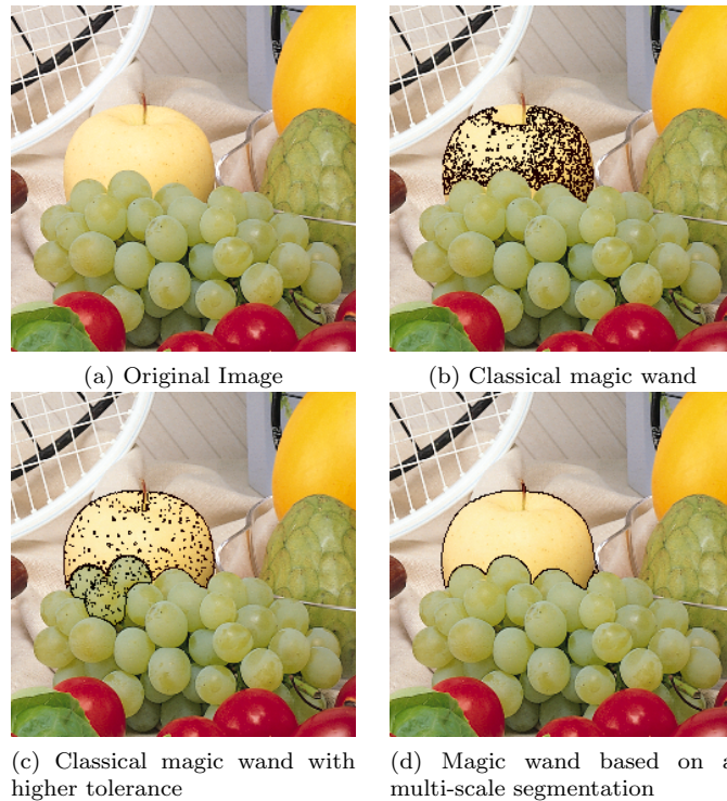
Figure 2. Comparison between the classical magic wand and the one combined with the multi-scale segmentation.
