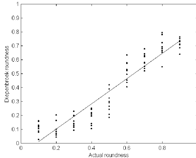
Figure 5. Relationship between Diepenbroek-computed roundness and actual roundness, with correlation of 0.94.
