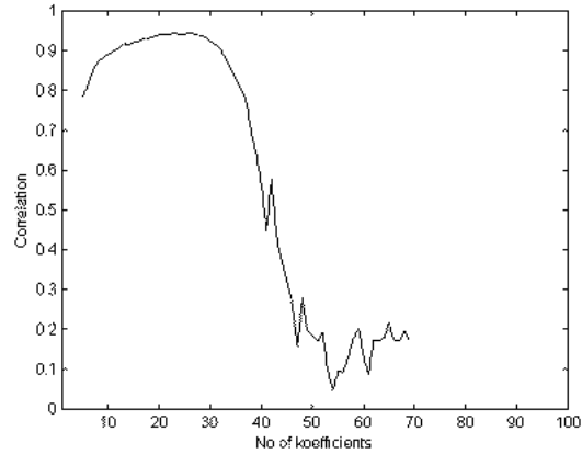
Figure 4. Correlation between the Diepenbroek and actual roundness values.
