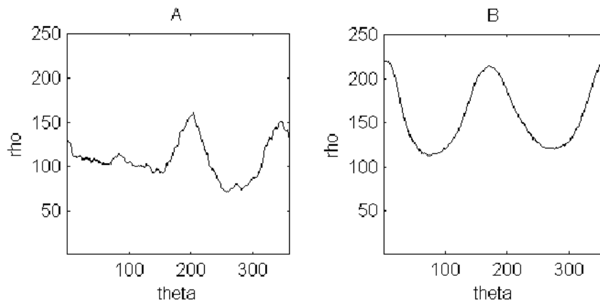
Figure 3. Polar coordinates of the rock fragments in Fig. 2.
