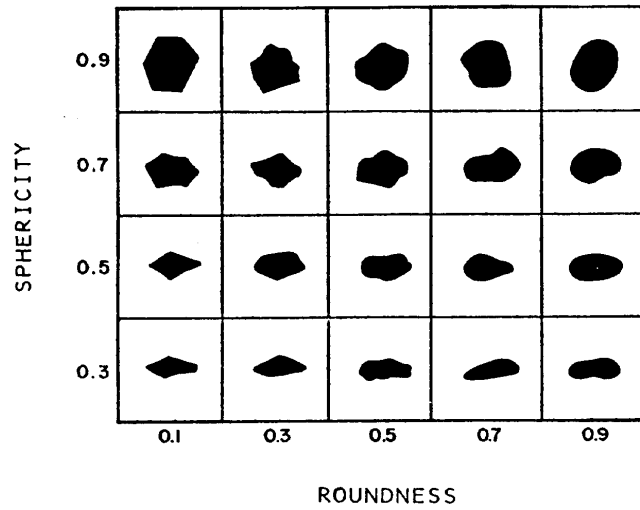
Figure 1. Subset of Krumbein particle roundness/sphericity chart.
