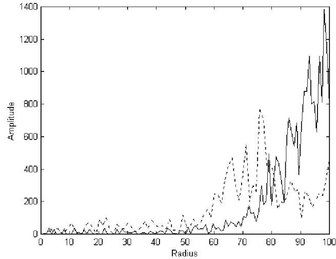
Figure 7. Granulometric curves (pattern spectra) of particle a (dotted line) and particle b (solid line) in Fig. 2. Radius is given as a percentage of the radius of the largest inscribed circle of each particle.
