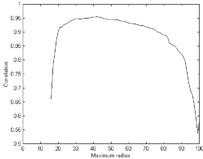
Figure 8. Correlation between the area removed through opening with a disk and the Krumbein roundness, as a function of disk radius, normalized between 0 and 100.
