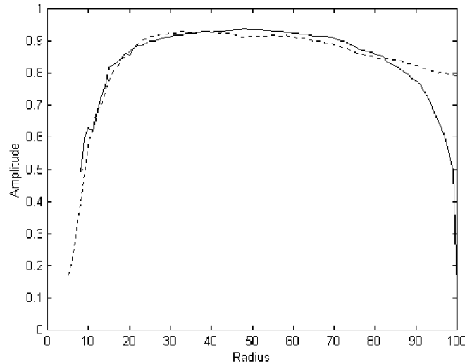
Figure 9. Correlation curves for method based on 1D opening of polar coordinate profile (dotted line), and method based on circular opening of particle shape. The curves are almost identical and exhibit excellent correlation values in the [30; 70] input range.
